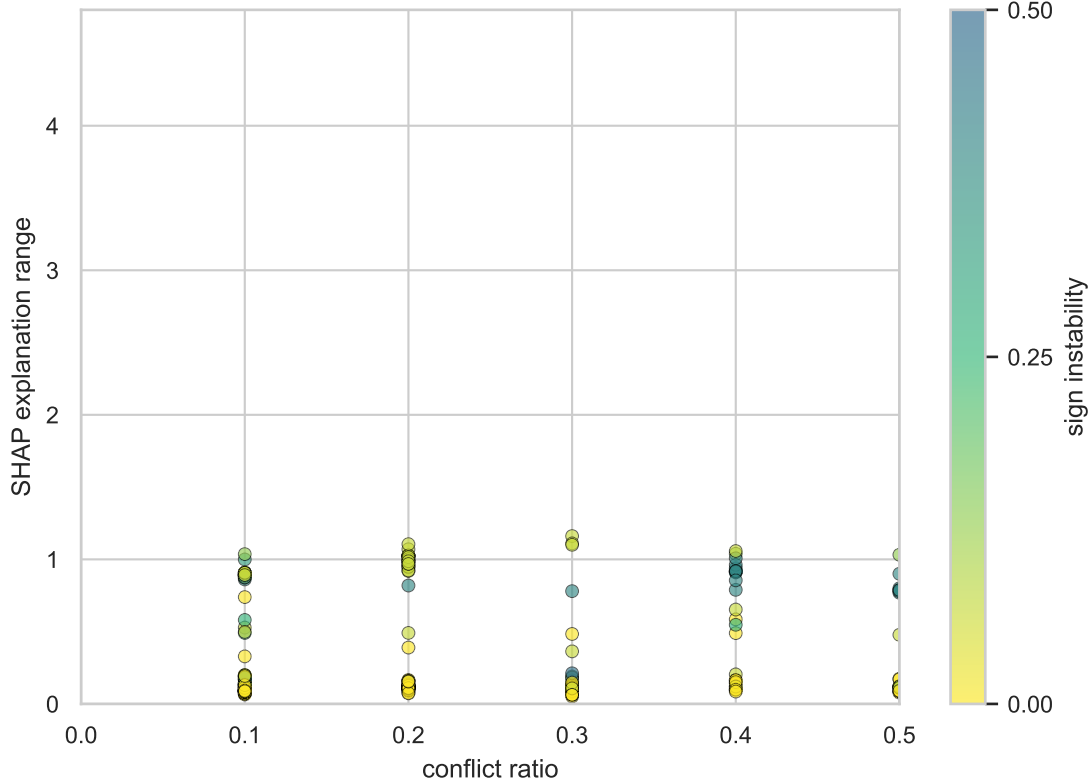
cat_protocol_type_tcp: SHAP explanation range (Spearman r = 0.108 )
